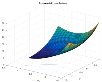
Figure: Exponential loss surface and the max-margin solution of SVM (line direction). By Matus Telgarsky . ICML 2013.
